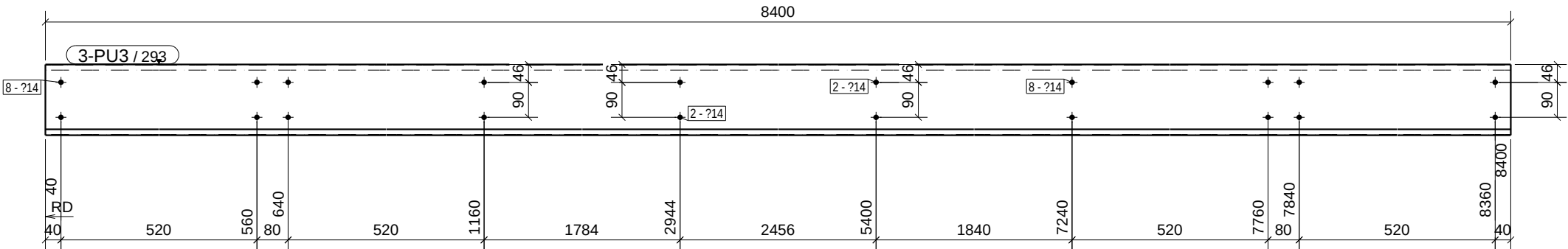
FRONT VIEW
